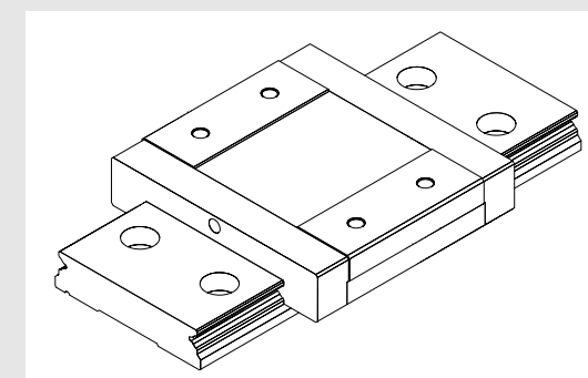
[SBMW type] The width and length of linear block and rail are modified to increase load ratings and permissible moments.
